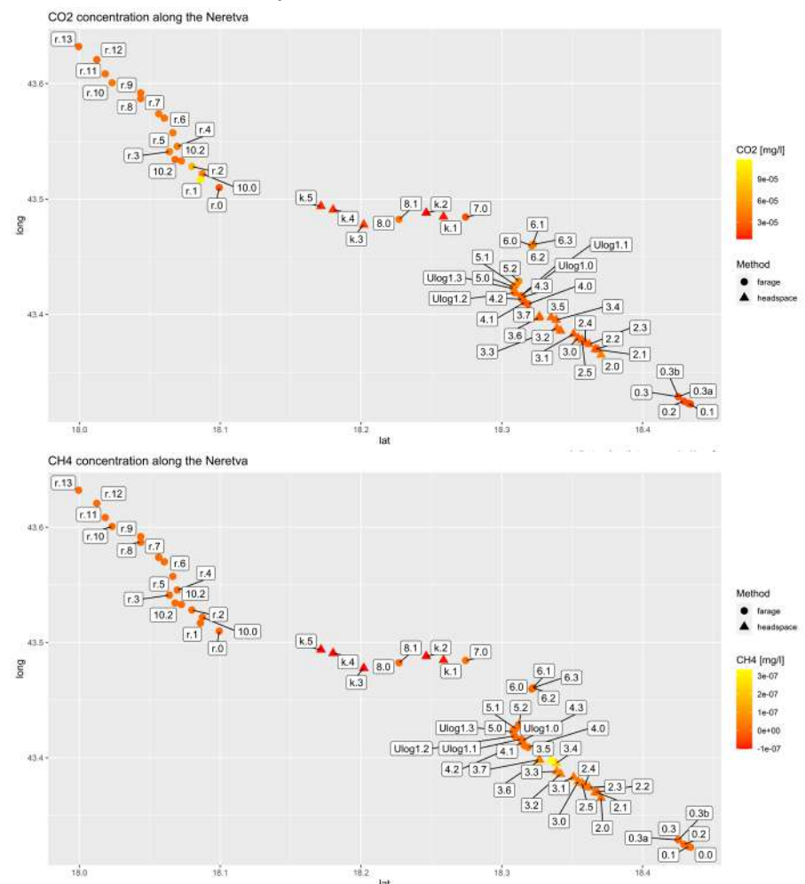
Figure 37 - This graph shows the \text{CO}_2 and \text{CH}_4 concentration (in mg/l) along the Neretva River, with a high variability along the measured continuum. The sites with the prefix "r." and "k." were not reachable by car or foot and therefore sampled via raft and kayak, respectively.
