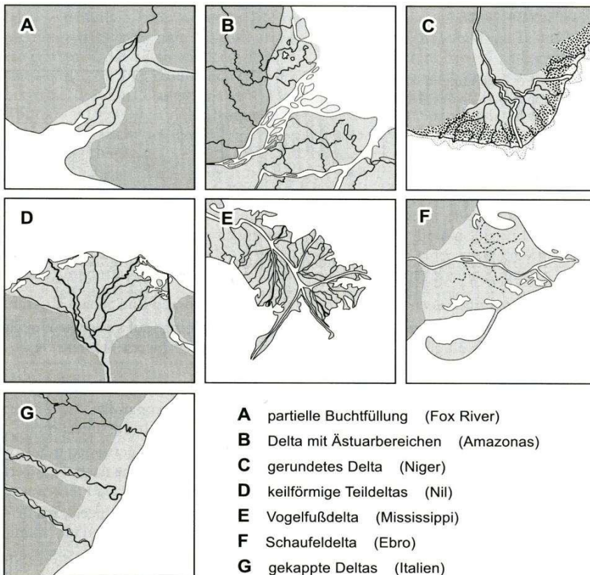
Figure 1: Types of deltas (from Ahnert 2001). The most common Mediterranean delta types are those shown in D, F and G. The Mediterranean deltas are generally river-sediment-driven and not predominantly wave-formed or tidal.
