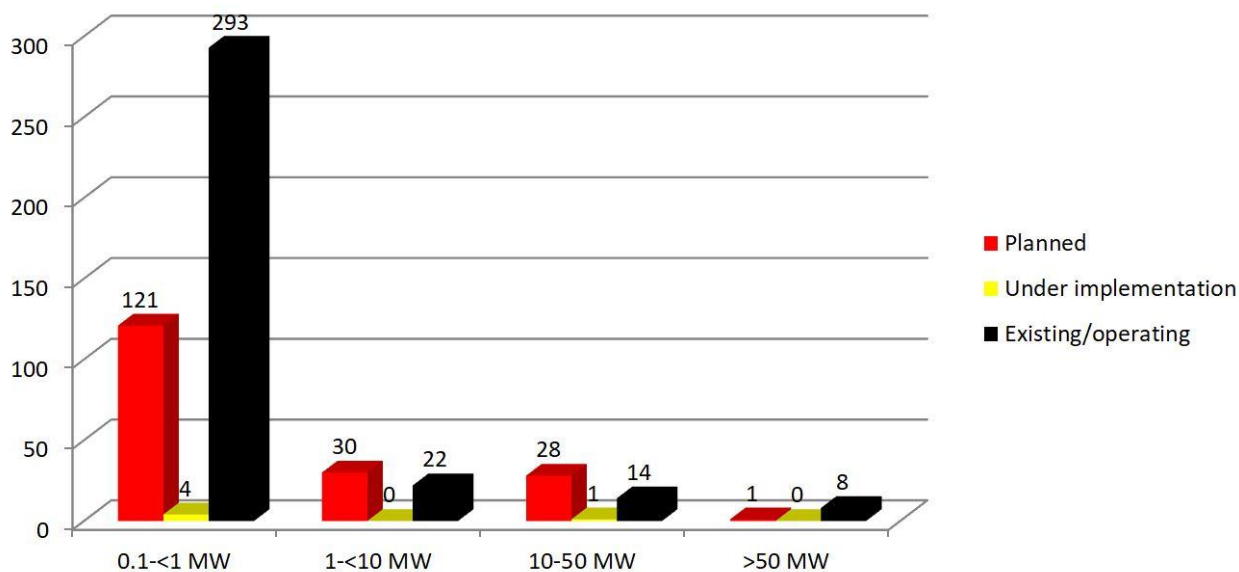
Hydropower Plants in Slovenia by size (capacity) 2017
